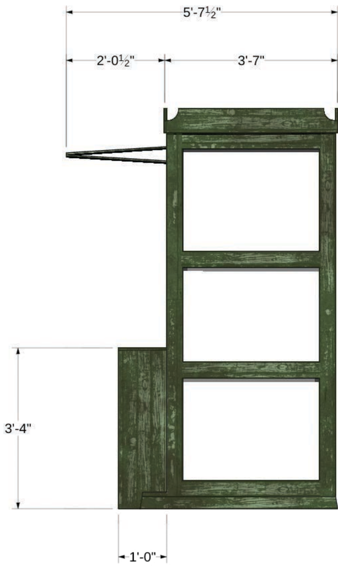
NEWSPAPER STAND SIDE VIEW (MIRROR OTHER SIDE)
