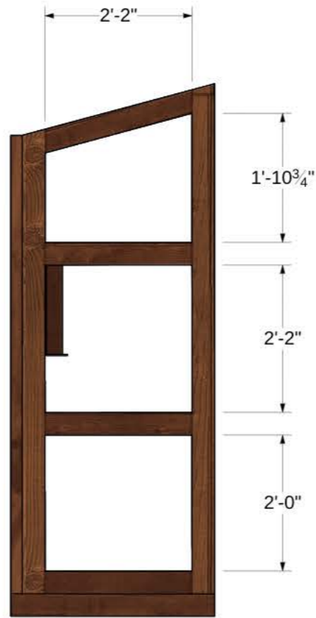
TELEPHONE BOOTH LEFT VIEW
