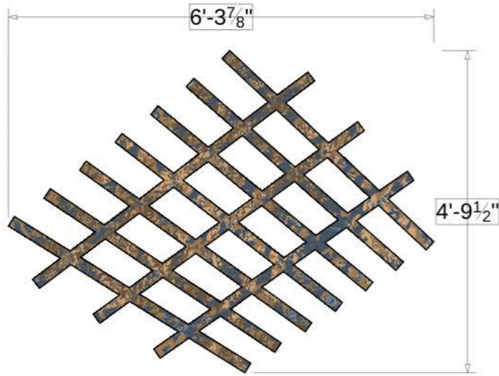
USR GRATE
