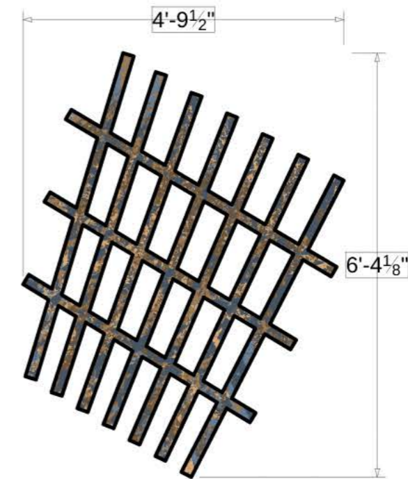
DSL GRATE
