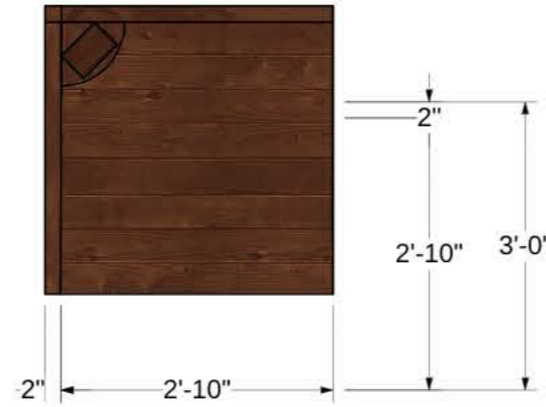
TELEPHONE BOOTH TOP VIEW
