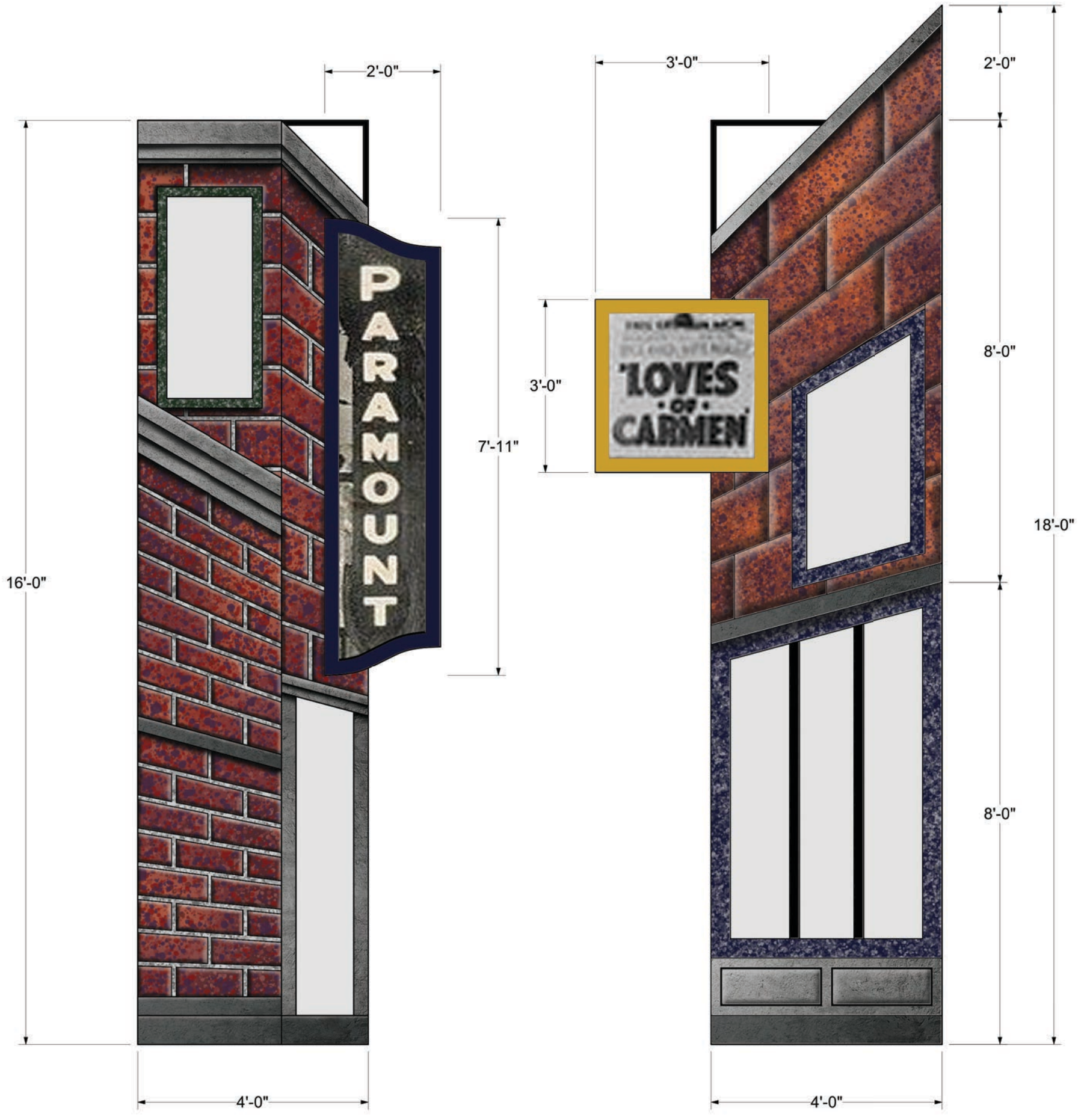
PORTAL 3 SR LEG
