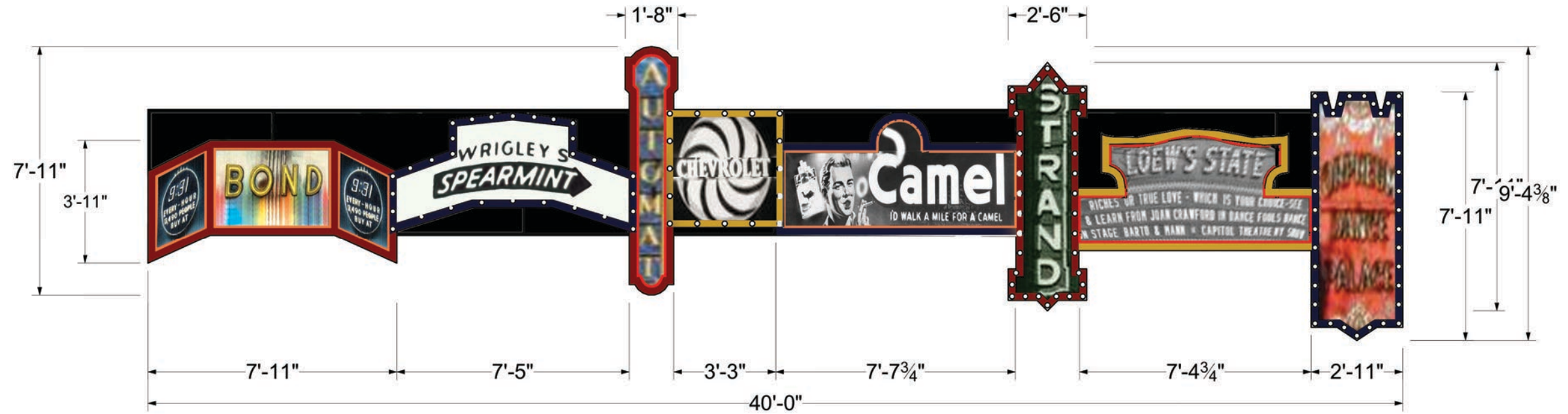
PORTAL 1 HEADER
