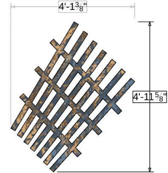
USL GRATE
