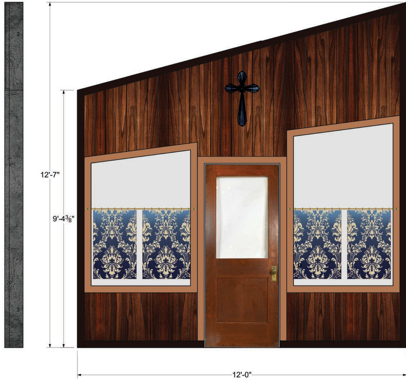
US BUILDING SWING WALL RIGHT VIEW
