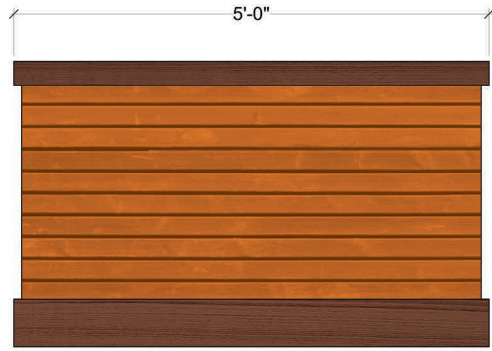
ASJ LOBBY COUNTER FRONT VIEW
