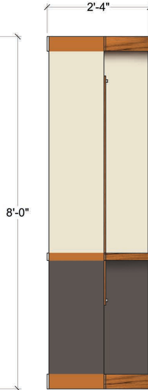
ROLLING WALL RIGHT VIEW
