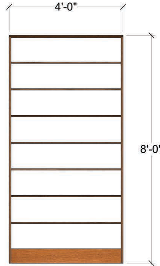
TOP BOOKCASE FRONT VIEW
