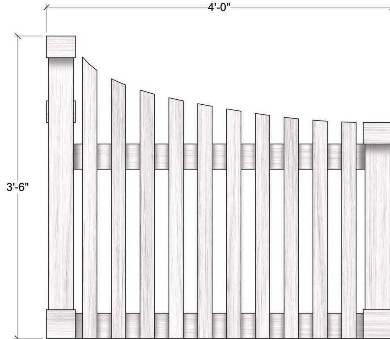
PICKET FENCE FRONT VIEW
