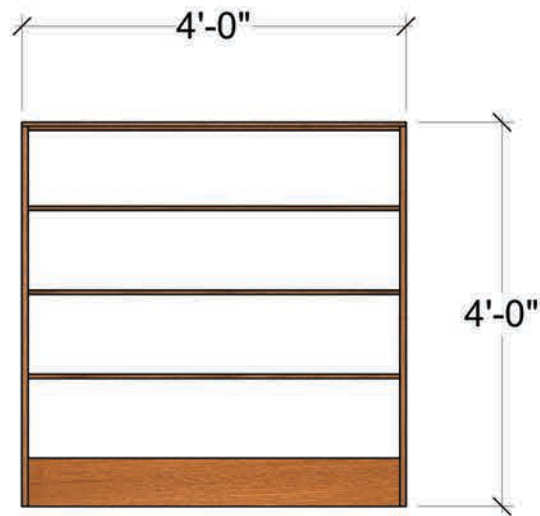
SHORT BOOKCASE FRONT VIEW
