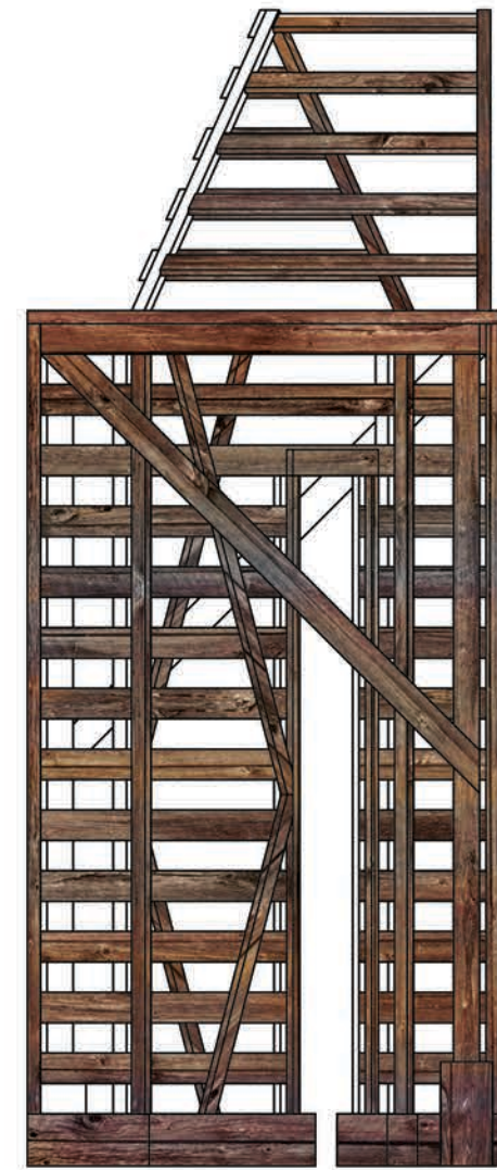
4'-6 3 / 8 " CABIN RIGHT VIEW
